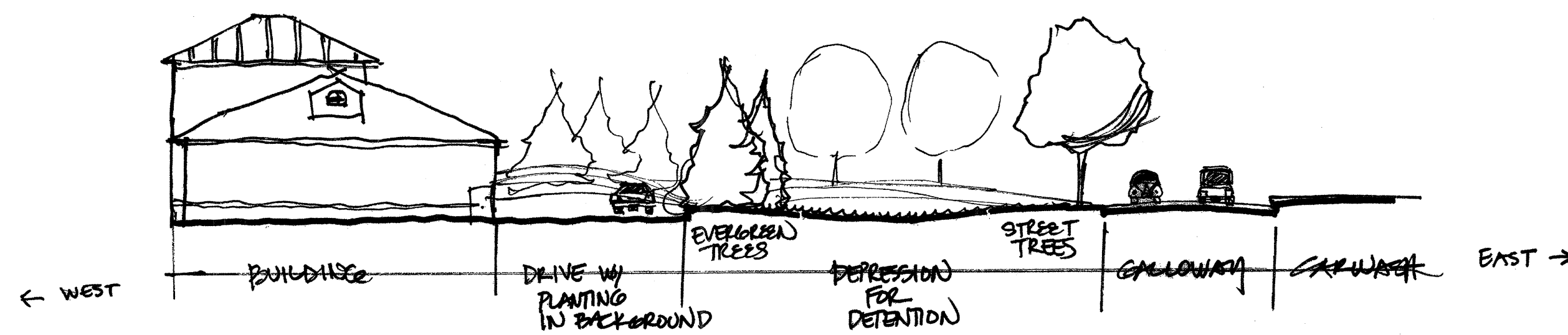
CROSS SECTION 2 FROM GALLOWAY LOOKING NORTH. 2.4.10
